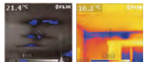
Insulation Alarm
